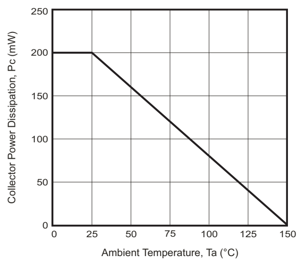
Fig.6 - P_c - T_a
