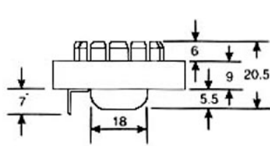
SIDE VIEW.1
