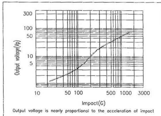
Output Voltage vs. Impact Response
