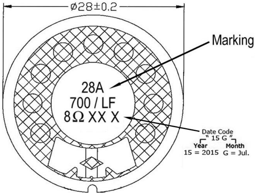
BOTTOM VIEW
