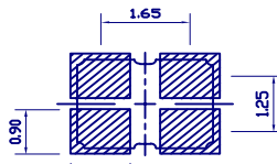
RECOMMENDED LAND PATTERN
