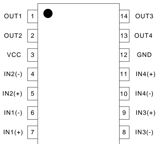
SOP-14
