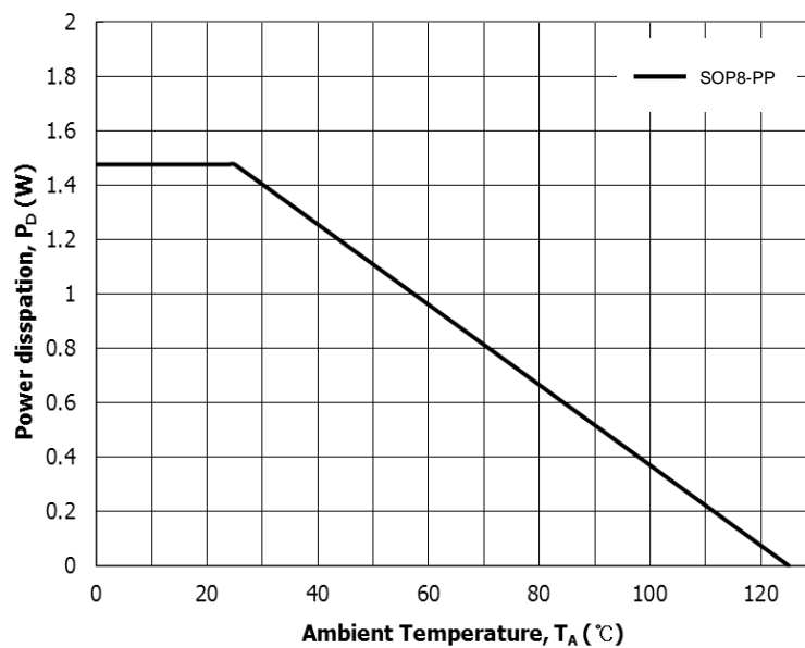
Power Dissipation( P_D ) vs. Ambient Temperature( T_A )
