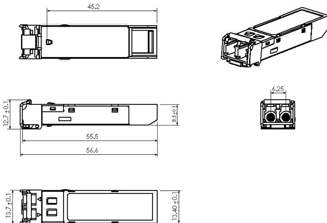
MSFP-1.25G-LX (dimensions are in inches)
