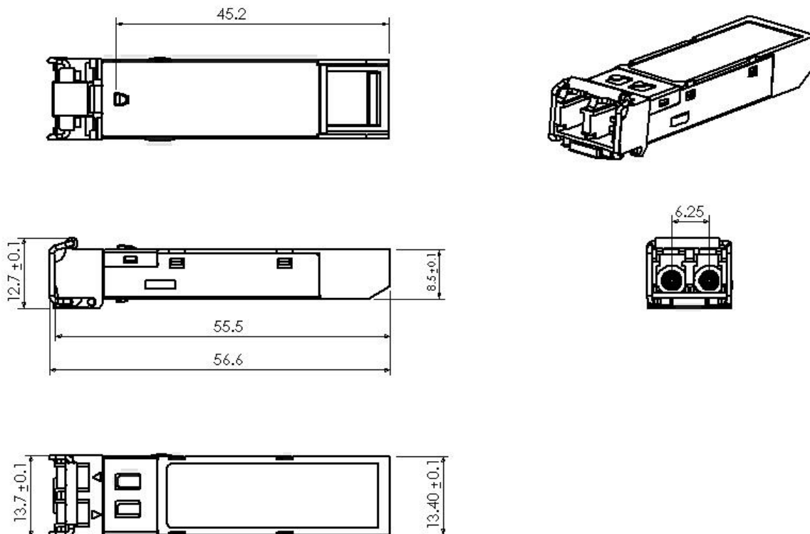
MSFP-1.25G-ZX (dimensions are in inches)
