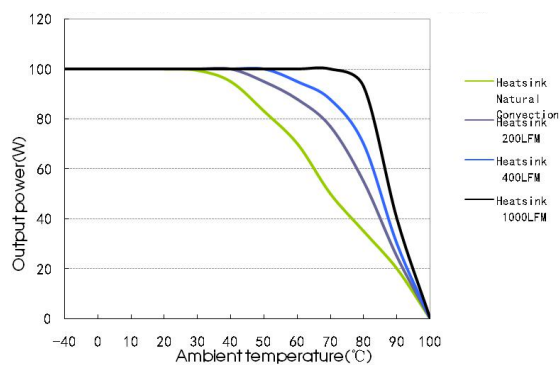
URF1D15QB-100WH Temperature Derating Curves (Vin=110V)
