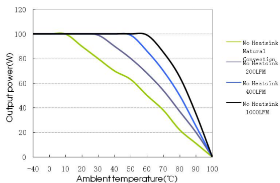
URF1D15QB-100W Temperature Derating Curves (Vin=110V)
