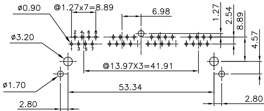
PCB Layout Component Side Shown
