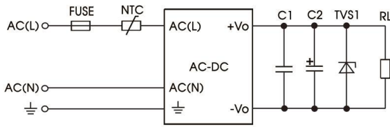
Fig. 1 LH**-10B**ER2(Single output)
