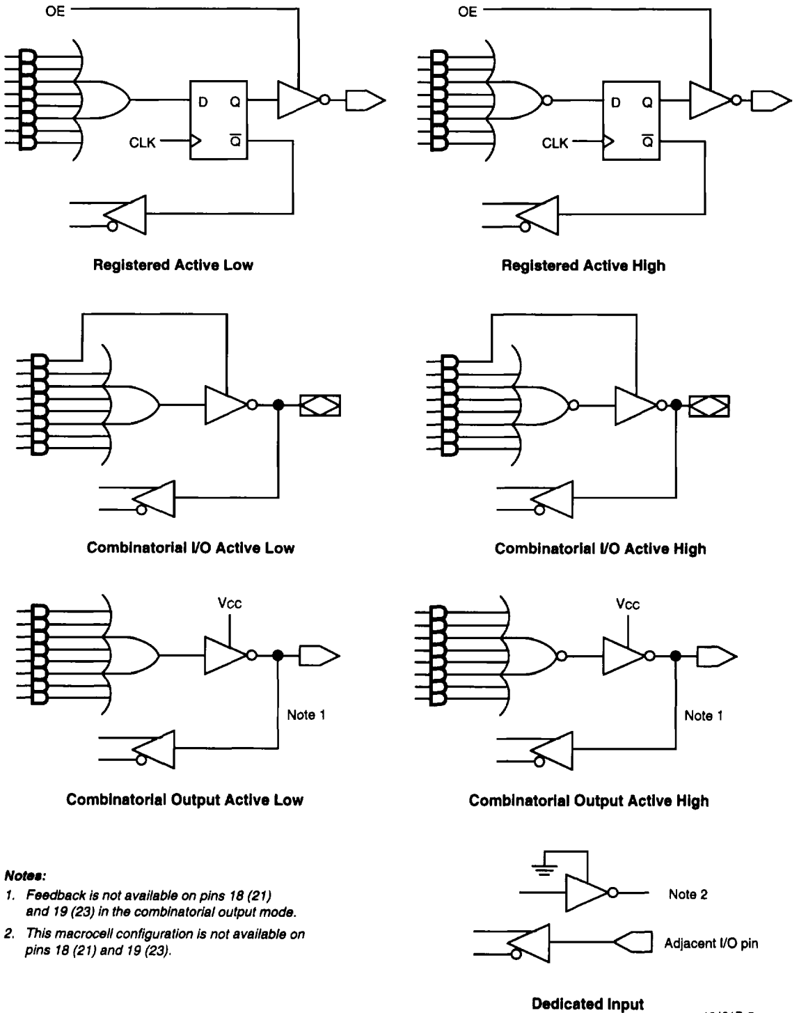
Figure 2. Macrocell Configurations
