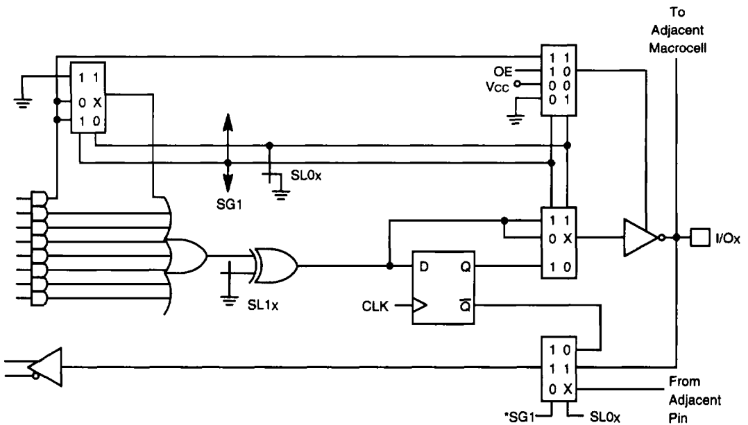
Figure 1. PALCE20V8 Macrocell
