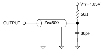
(Fig. 2) AC Output Load Circuit
