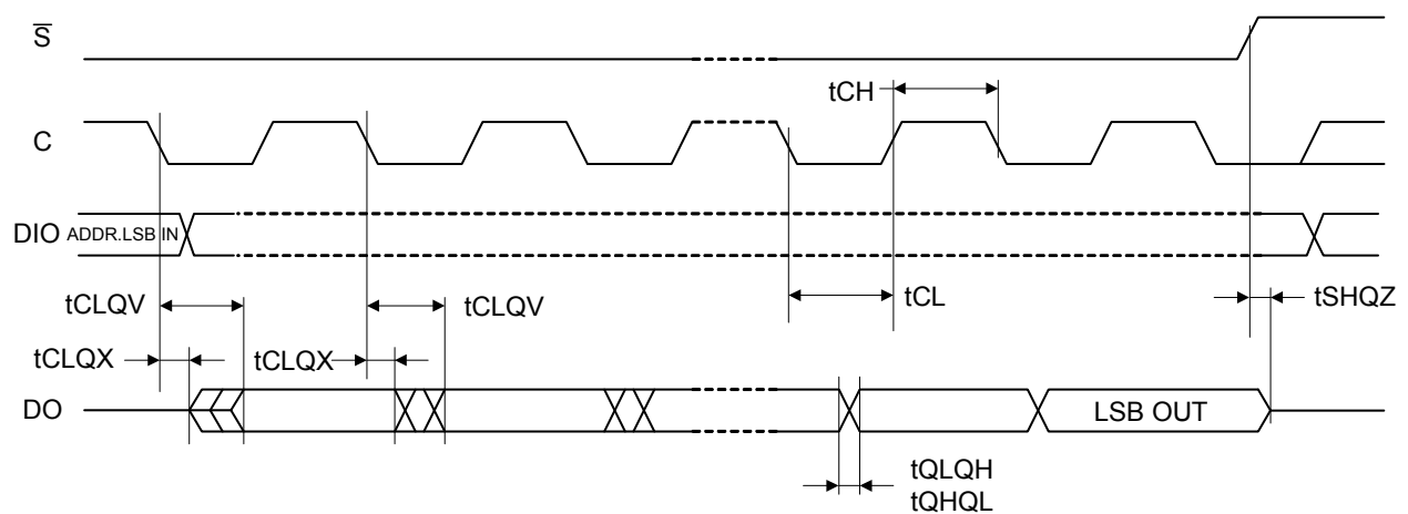
Figure 28. Output Timing
