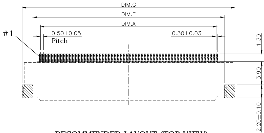
RECOMMENDED LAYOUT (TOP VIEW) GENERAL TOLERANCE: ±0.05mm
