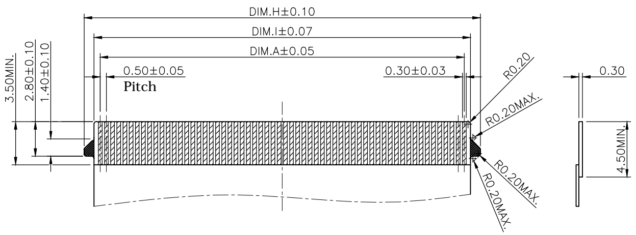
FPC LAYOUT
