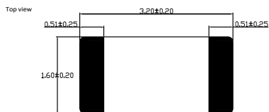
Dimensions (unit: mm)
