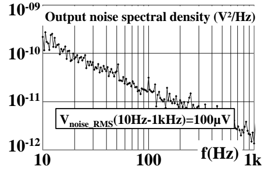
Figure 8: S_{\text{Vout}}(\text{V}^2/\text{Hz}) @25°C, I_{\text{Load}}=100\text{mA}
