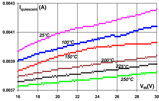
Figure 7: I_{\text{Quiescent}} vs. V_{\text{in}} over T^\circ
