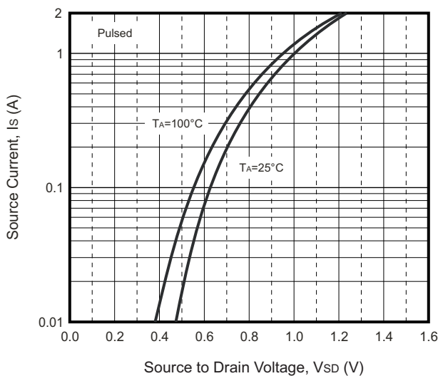
Fig.5 - I_S — V_{SD}
