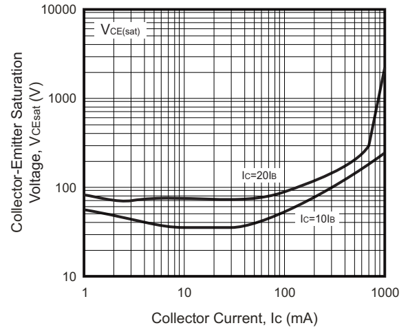
Fig.2 - Saturation Voltage vs. Collector Current
