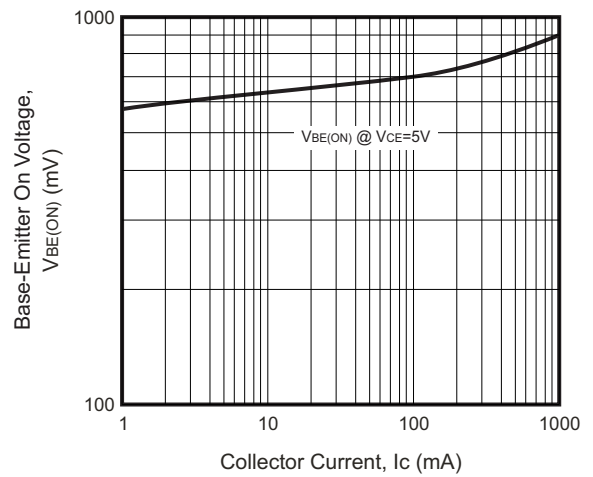
Fig.4 - On Voltage vs. Collector Current
