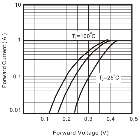
Fig. 3 - Forward Characteristics
