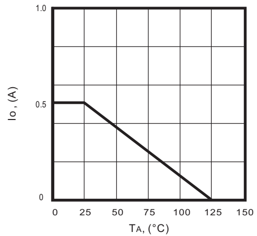
Fig.4 - Derating curve
