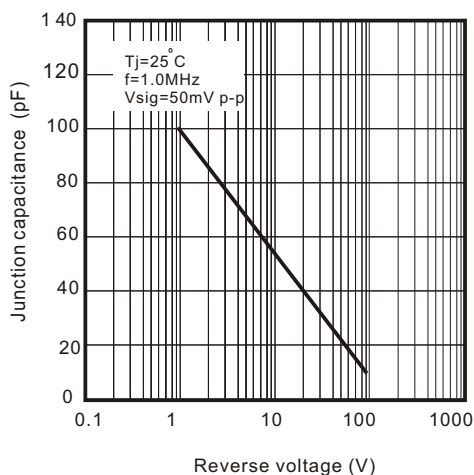
Fig. 3 - Junction capacitance
