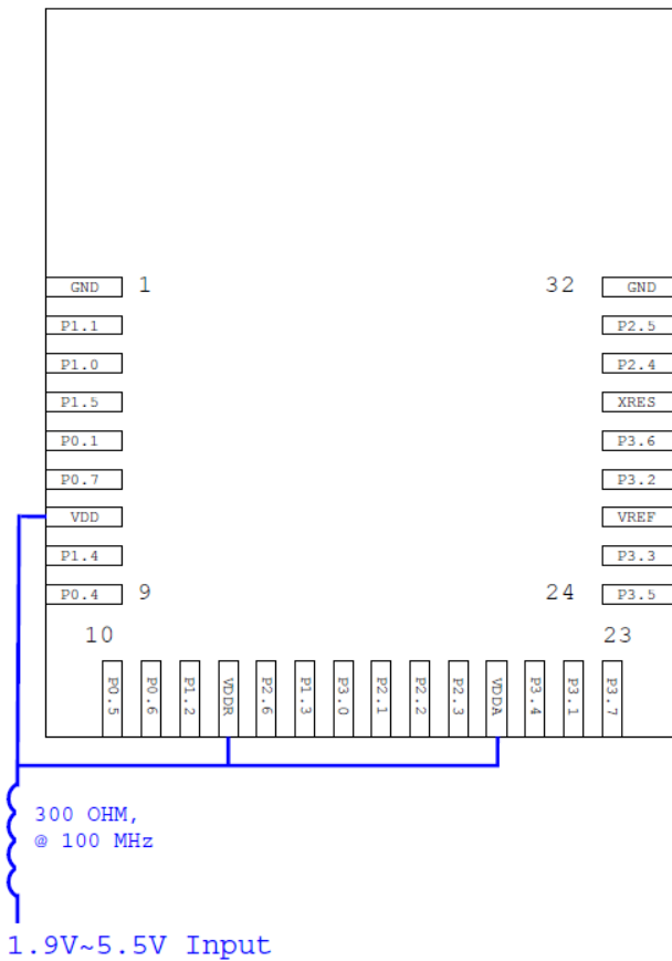
Single Ferrite Bead Option
