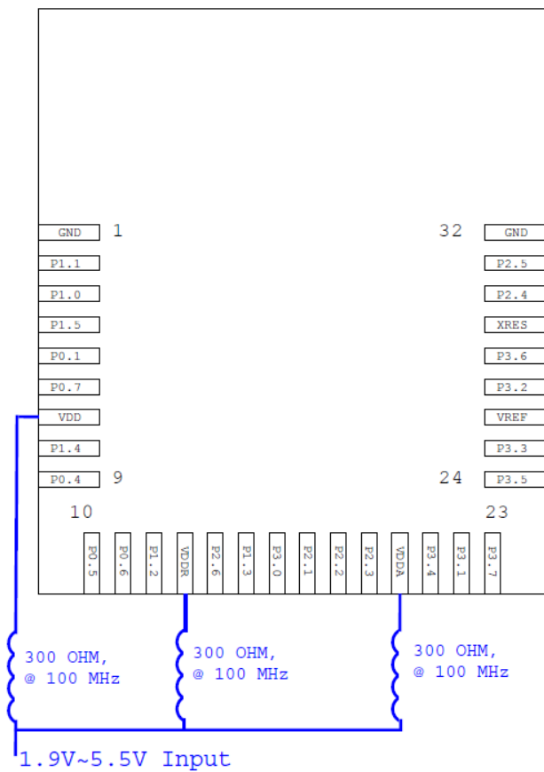
Three Ferrite Bead Option
