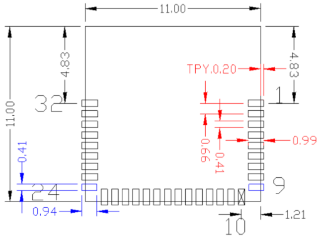
Figure 4. Host Layout Pattern for CYBLE-214015-01
