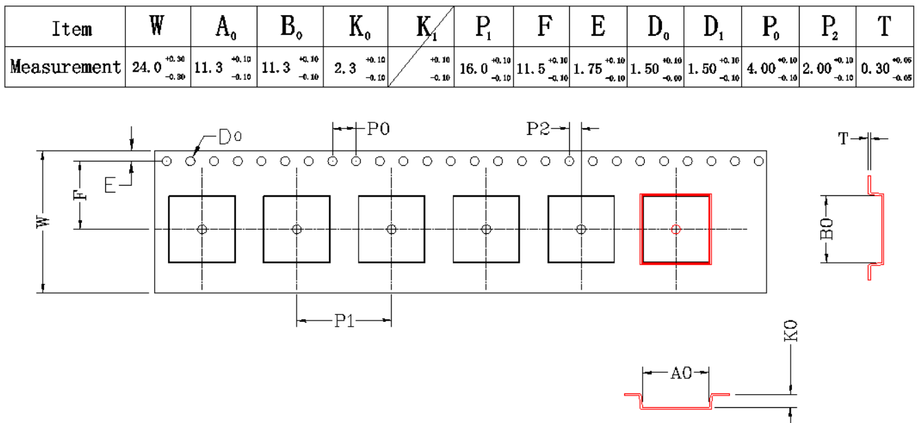
Figure 10. CYBLE-214009-00 Tape Dimensions
