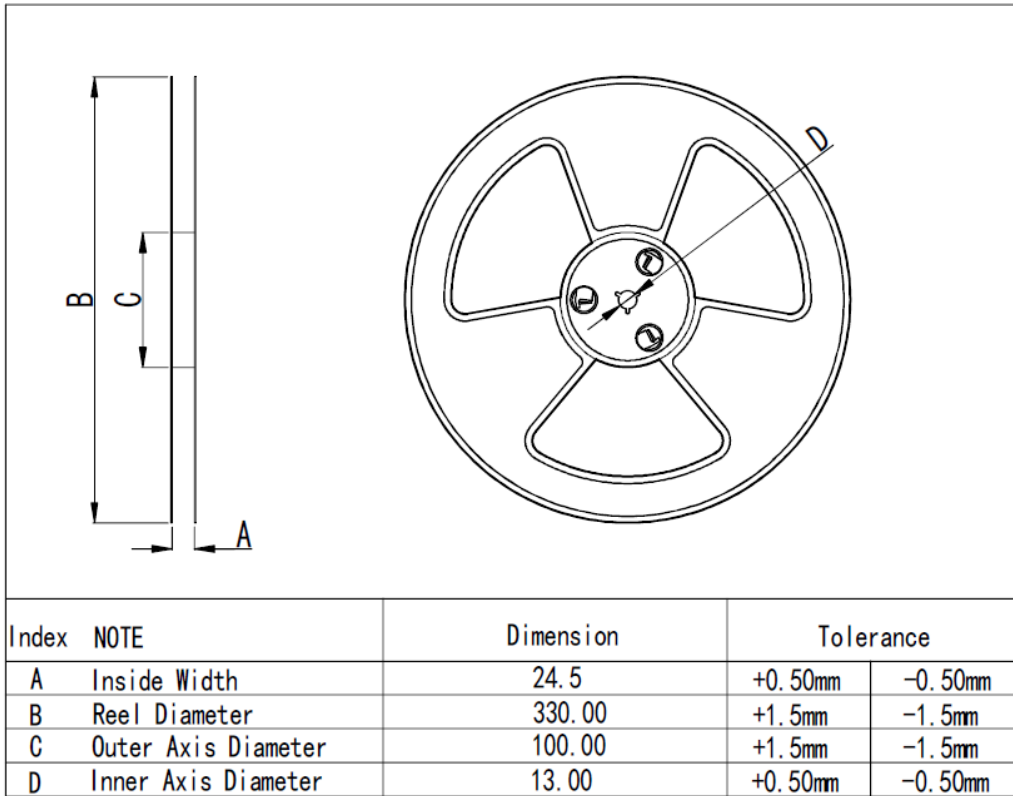
Figure 12. Reel Dimensions
