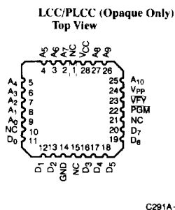
Figure 1. Programming Pinouts
