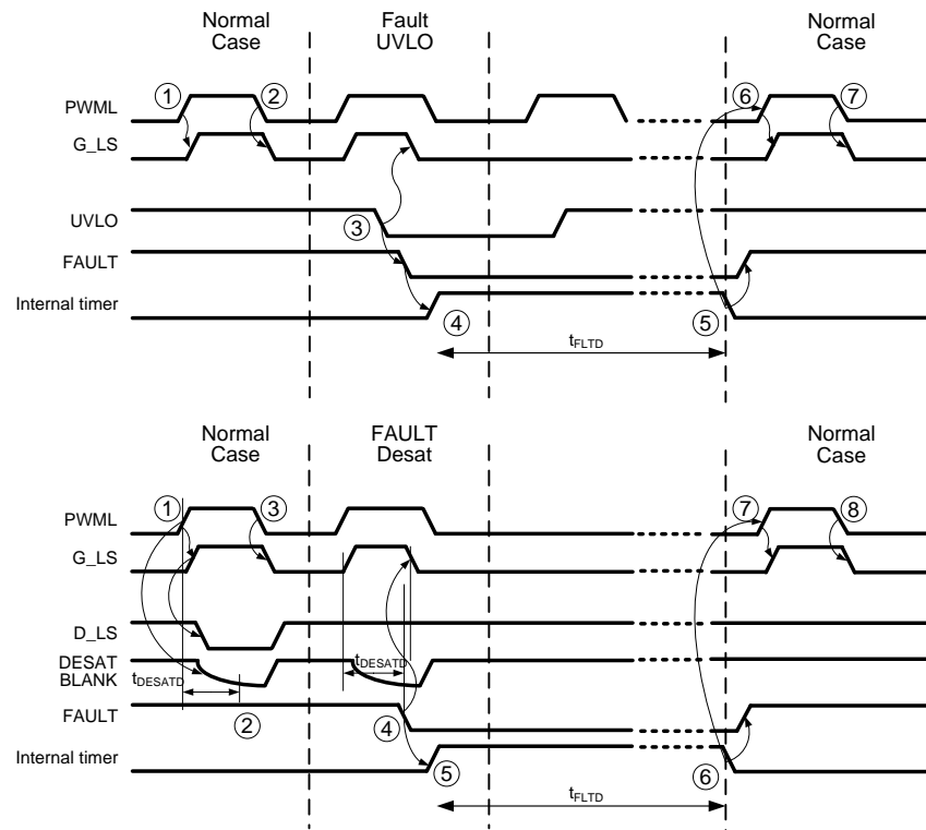
Figure 2: Timing diagram CMT-TIT8243/8244 low-side driver behaviour
