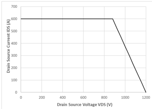
Figure 14 : Reverse Bias Safe Operating Area (RBSOA)
