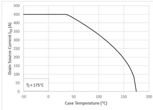
Figure 15: Continuous Drain Current Derating vs Case temperature
