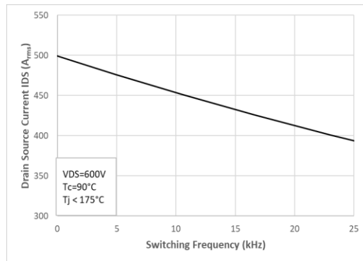
Figure 17 : Typical Output Current Capability vs Switching Frequency (Inverter Application)
