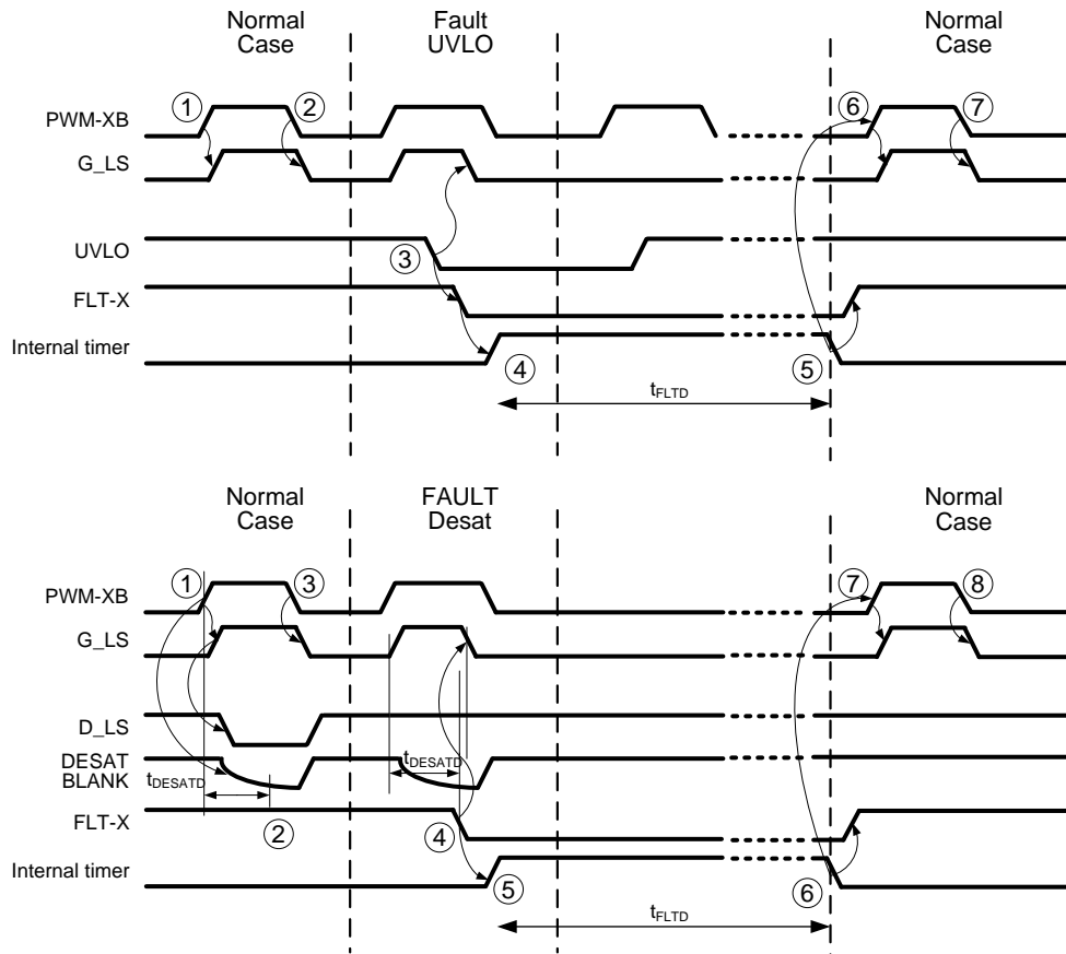
Figure 19: Timing diagram CXT-PLA3SA12450 low-side gate driver behaviour
