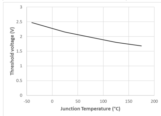
Figure 9: Threshold voltage vs temperature ( I_{DS}=20\text{mA} ; V_{GS}=V_{DS} )
