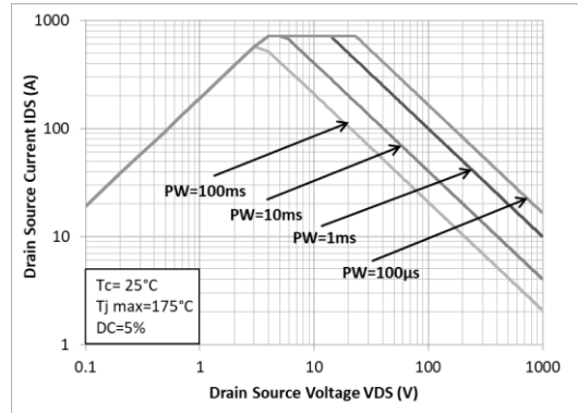
Figure 13: Forward Bias Safe Operating Area (FBSOA)
