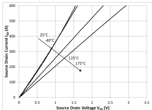
Figure 5: 3rd quadrant characteristics ( V_{GS}=15V , t_p < 200\mu s ) 6
