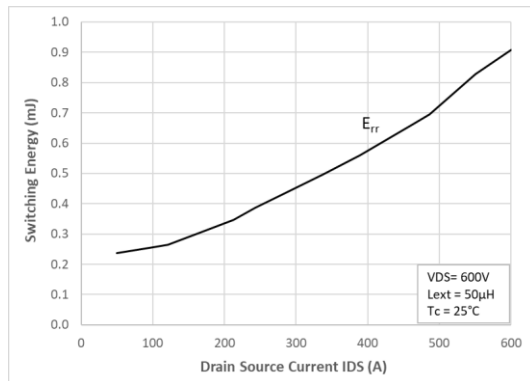
Figure 11 : Reverse Recovery Energy vs Drain Current
