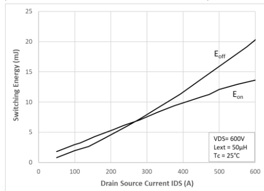
Figure 10 : Switching Energy vs Drain Current
