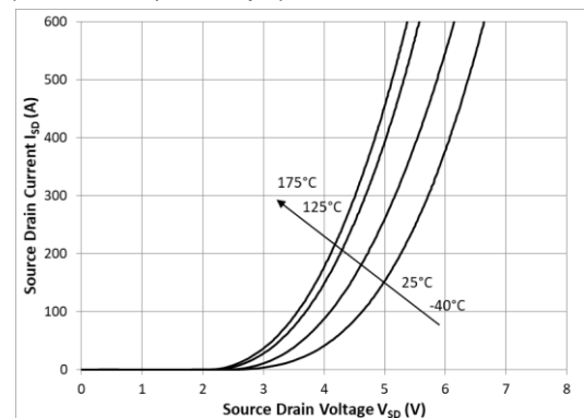
Figure 6: 3rd quadrant characteristics ( V_{GS}=-3V , t_p < 200\mu s ) 6
