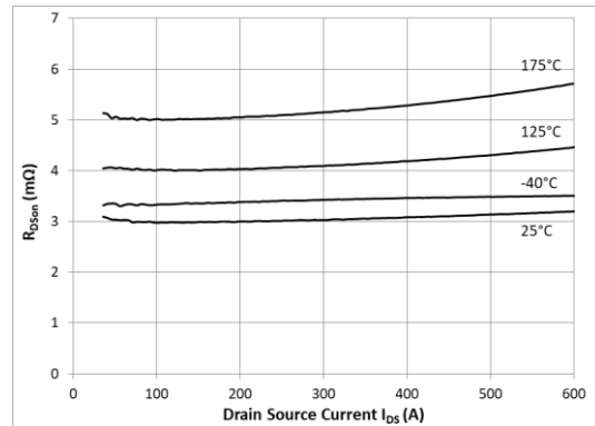
Figure 2: On-state drain source resistance vs. Drain current ( V_{GS}=15V , t_p < 200\mu s ) 6
