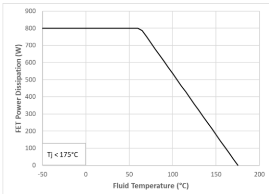
Figure 16 : Maximum Power Dissipation Derating vs Case temperature
