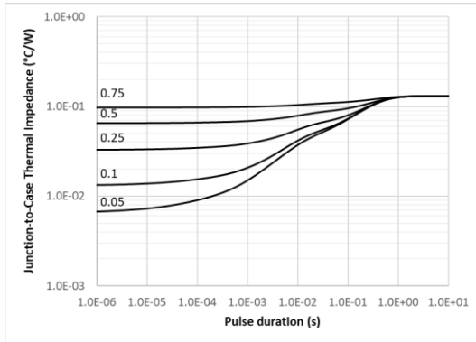
Figure 12: MOSFET Junction to Case Thermal Impedance
