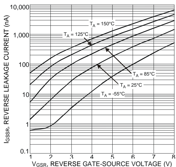
Fig. 12 Reverse Gate-Source Leakage Current vs. Voltage
