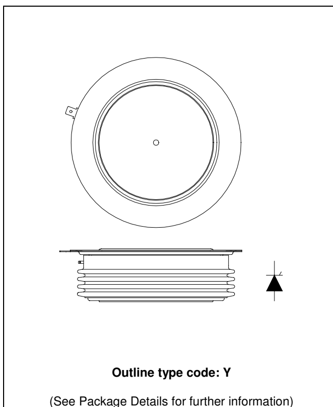
Fig. 1 Package outline
