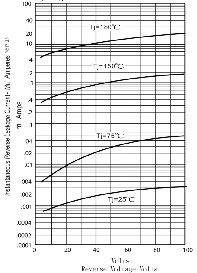
Figur.4-Typical Reverse Characteristics
