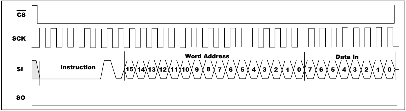
Figure 5-7. WRITE Timing
