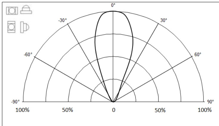
Relative Sensivity VS. Angular Displacement
