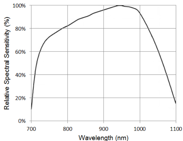
Spectral Sensitivity
