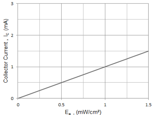
Collector Current VS. E_e
