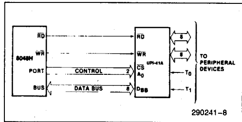
Figure 2. 8048-8741A Interface
