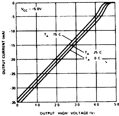
Output Current vs. Output "HIGH" Voltage
