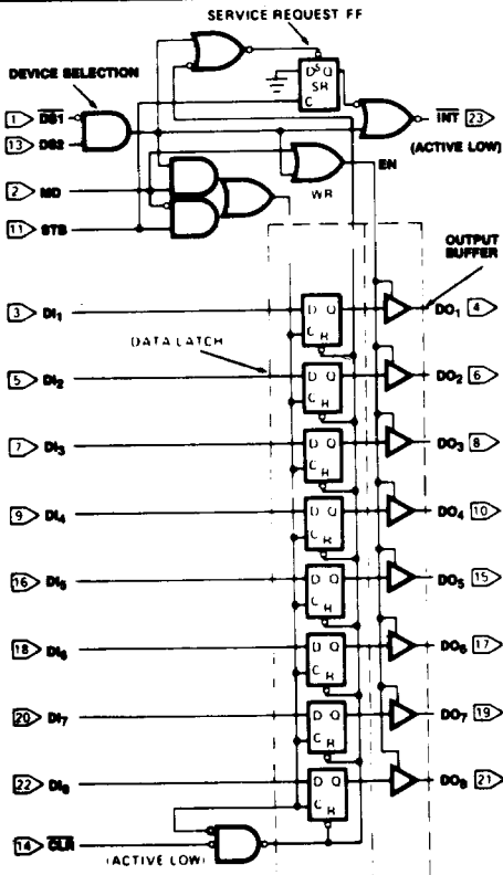
Figure 1. Logic Diagram
