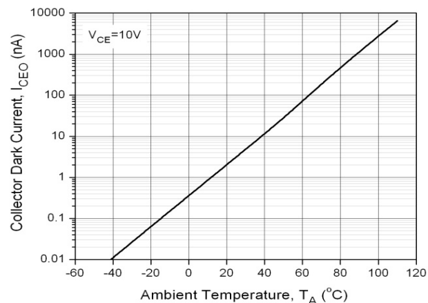
Fig 6 Collector Dark Current vs T_A
