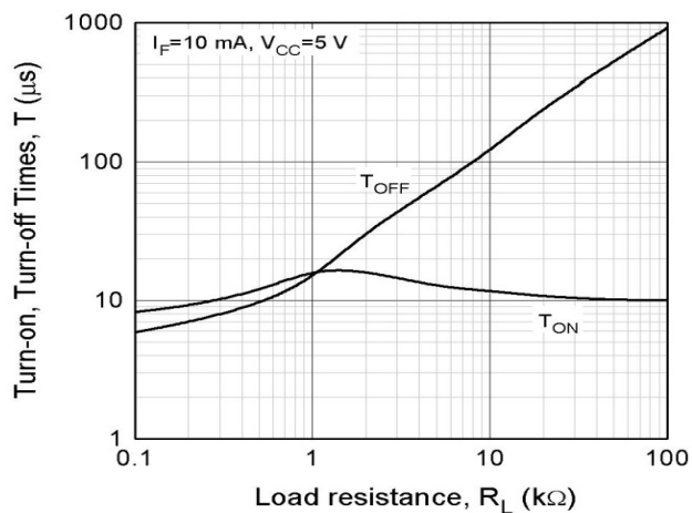
Fig 7 Turn-On and Turn-Off Times vs Load Resistance
