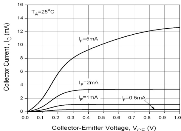
Fig 2 Collector Current vs Collector-emitter Voltage (2)
