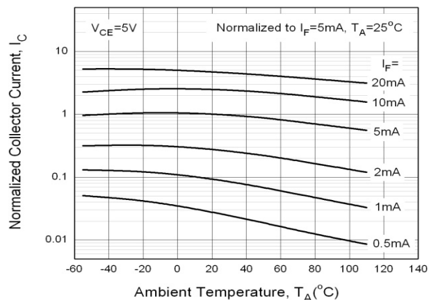
Fig 4 Normalized Collector Current vs T_A
