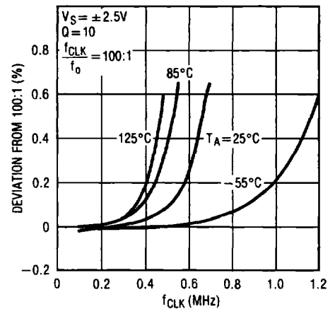
Graph 12. Mode 1: (f CLK /f 0 ) vs f CLK and Temperature
