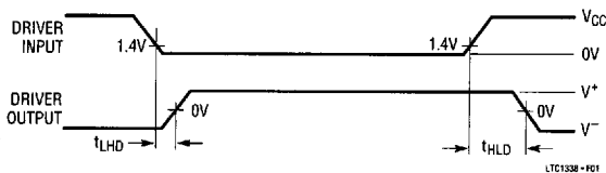
Figure 1. Driver Propagation Delay Timing
