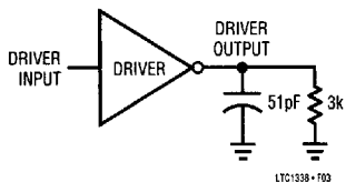
Driver Timing Test Load
