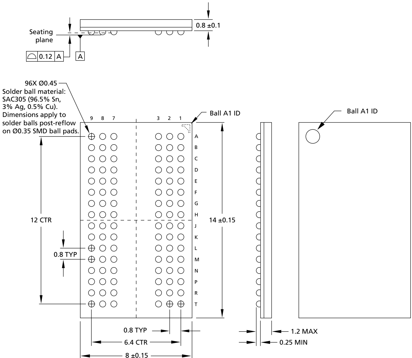
Figure 13: 96-Ball FBGA – x16 (JT)
