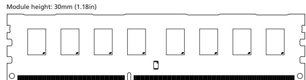
Figure 1: 240-Pin UDIMM (MO-269 R/C A)
