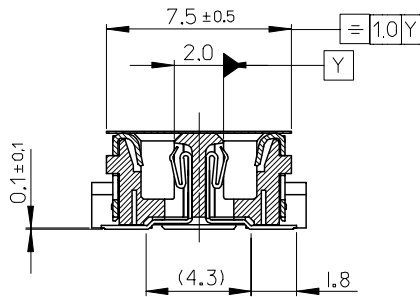
SECTION A-A 5-1
