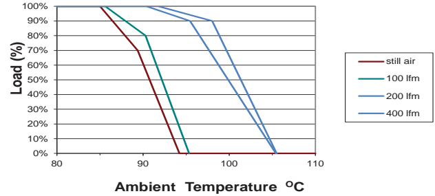
NCS1S2403SC
