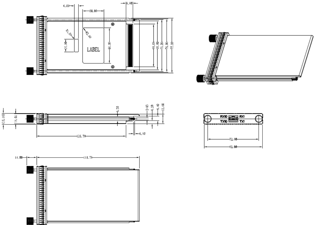
Figure9. Mechanical Specifications
