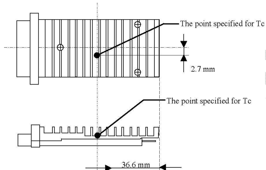
Figure 1 Mechanical dimensions
