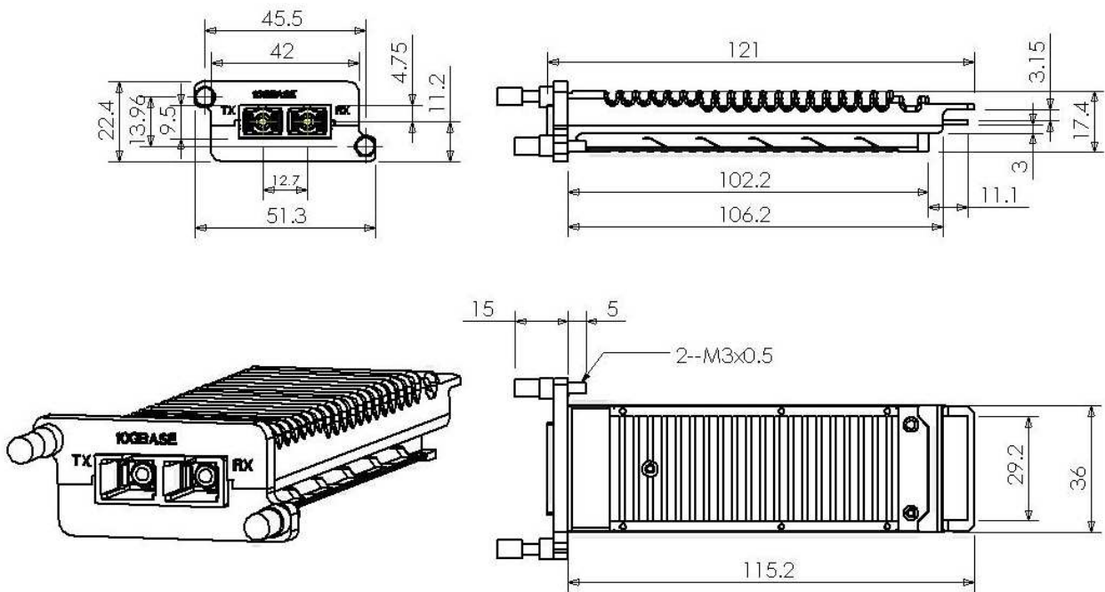
Figure 1 Mechanical dimensions
