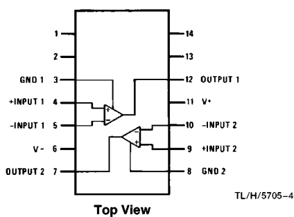
Dual-In-Line-Package
