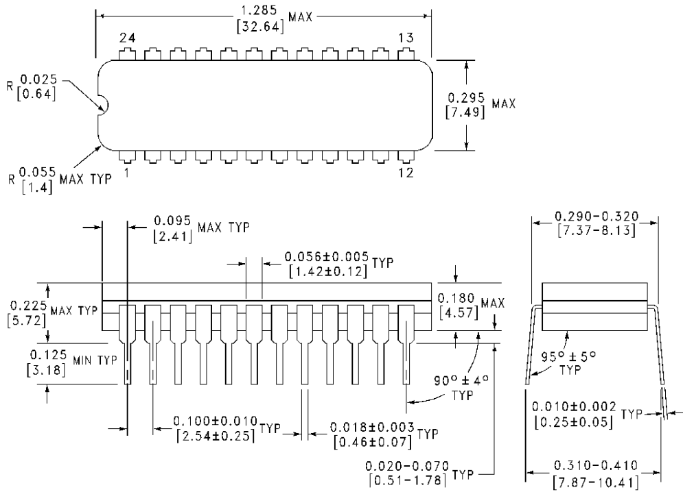
Cavity Dual-In-Line Package (J) NS Package Number J24F
