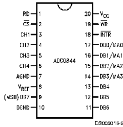
Dual-In-Line Package
