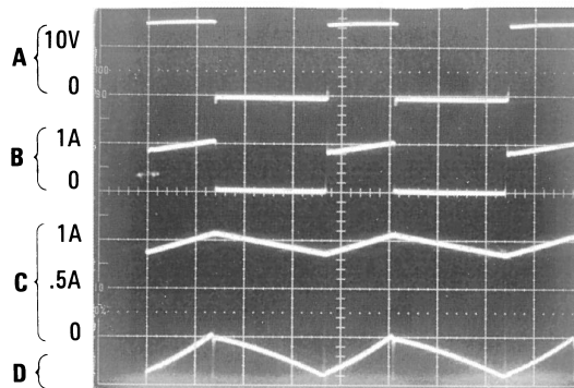
Switching Waveforms
