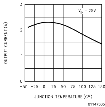
Current Limit
