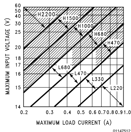
FIGURE 5. LM2575(HV)-12
