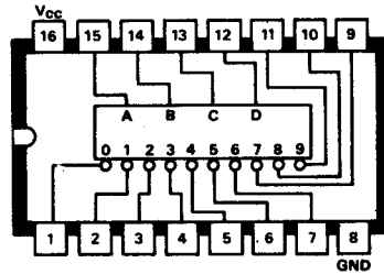
B35 SN7444N Excess-3-gray-to-Decimal decoder
